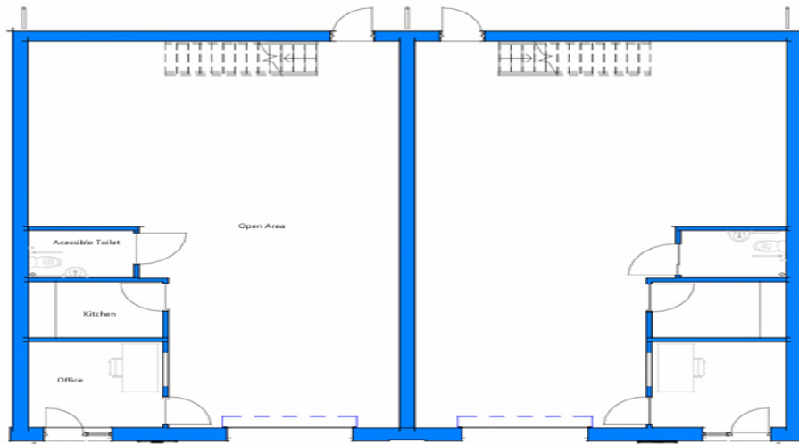
Proposed Ground Floor Plan - Units 1, 2, 3, 4, 7, 8 1 : 100
